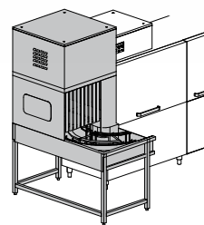
EVO: DRA184MC 4,5 kW Electric DRA189MC 9 kW Electric PRO: DRA184MT 4,5 kW Electric DRA189MT 9 kW Electric DRA18VMT Steam Asciugature ad angolo a 180° Dryer with arc 180°
